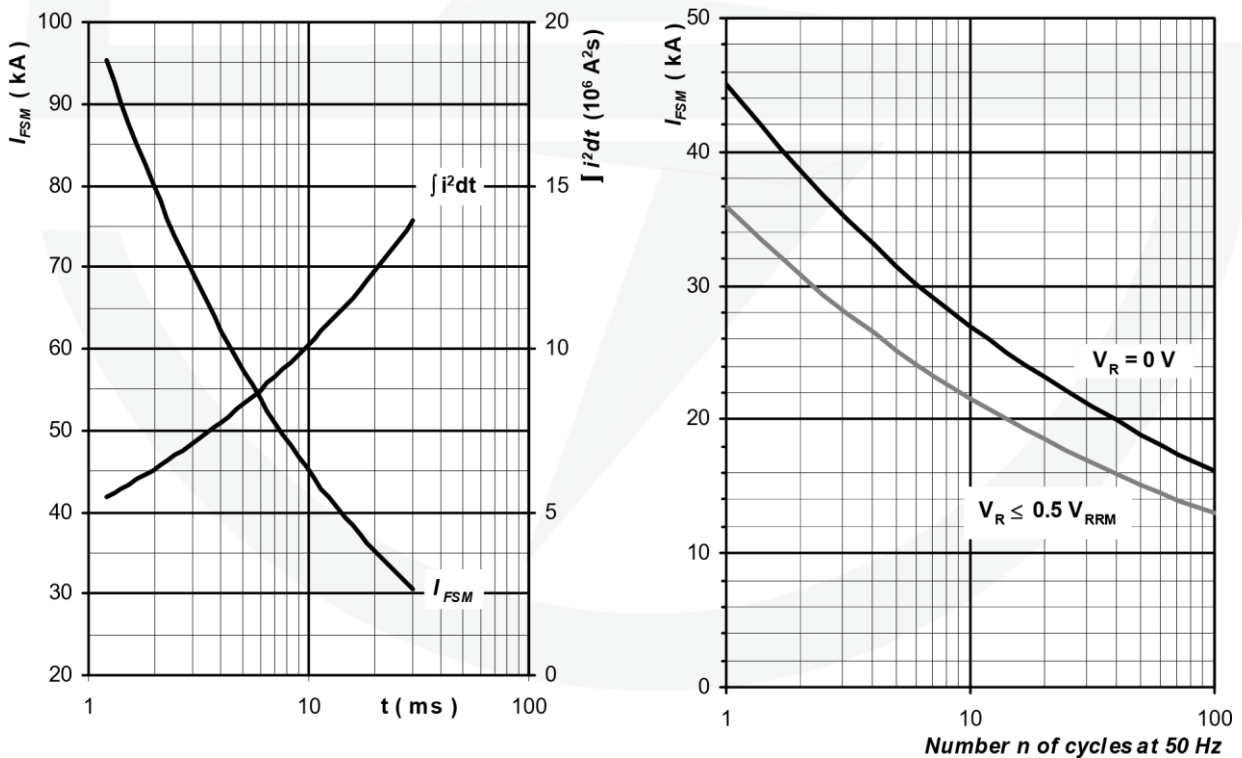
Fig. 4 Surge forward current vs. pulse length, Fig. 5 Surge forward current vs. number half sine wave, single pulse, of pulses, half sine wave, T_j = T_{jmax} V_R = 0 \text{ V} , T_j = T_{jmax}
