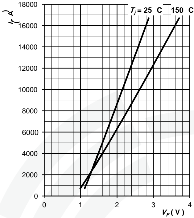
Fig. 3 Maximum forward voltage drop characteristics
