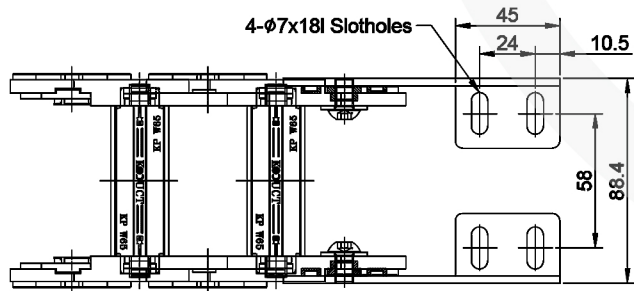
VIEW-B FIXED END (S=2:1)
