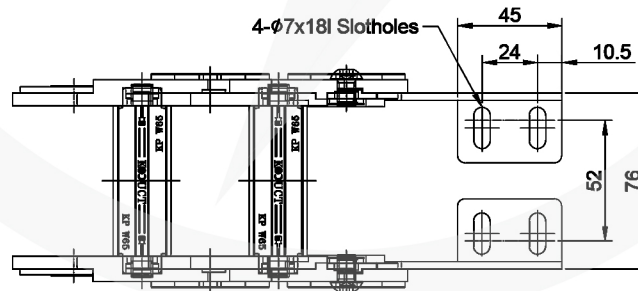
VIEW-C MOVING END (S=2:1)
