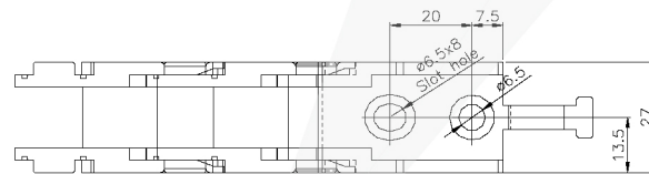
VIEW-C MOVING BRACKET(S=2:1)
