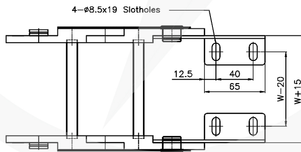
VIEW-C MOVING END (S=2:1)
