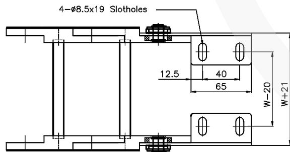
VIEW-B FIXED END (S=2:1)
