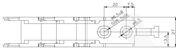
VIEW-B FIXED BRACKET(S=2:1)
