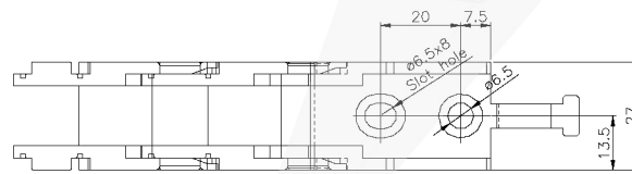
VIEW-C MOVING BRACKET(S=2:1)
